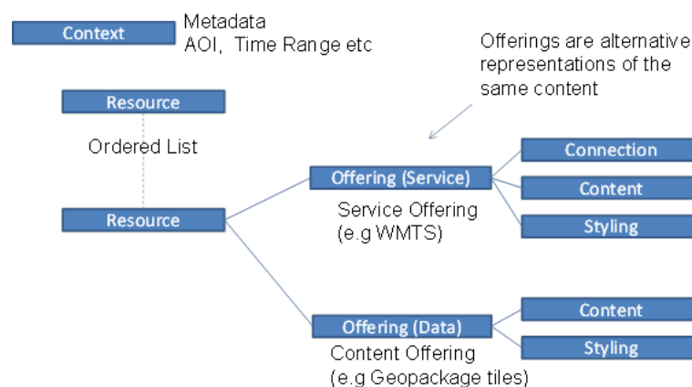
Figure 12 - Structure of an OWS Context document
